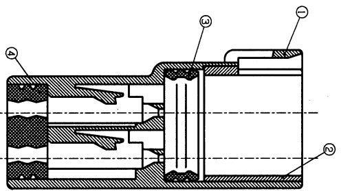
SECT. A-A
